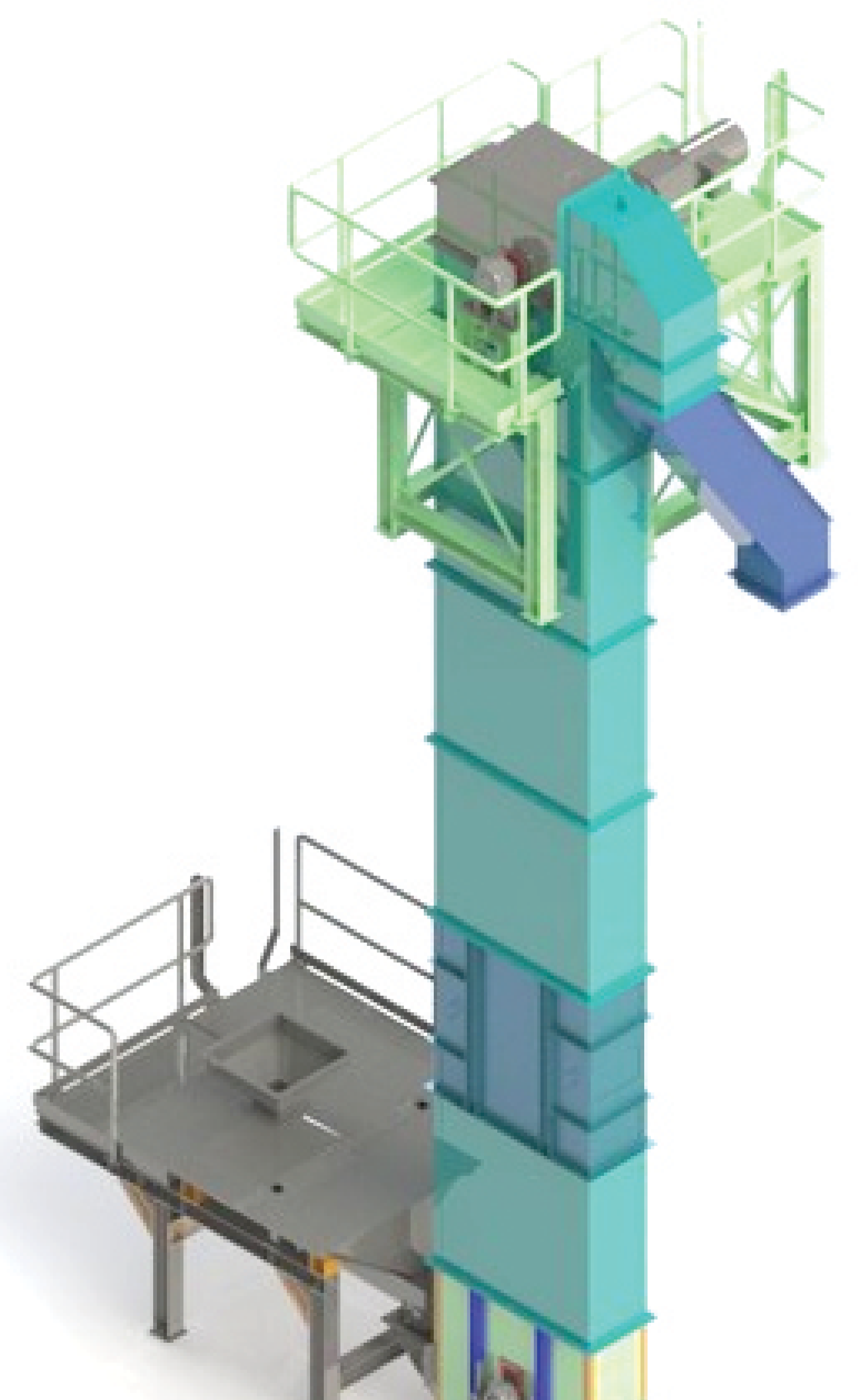
Bucket Elevator
