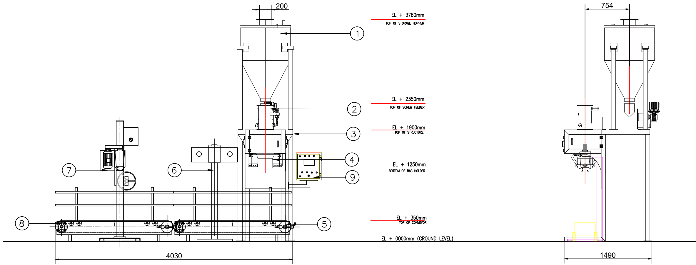
ELEVATION VIEW
